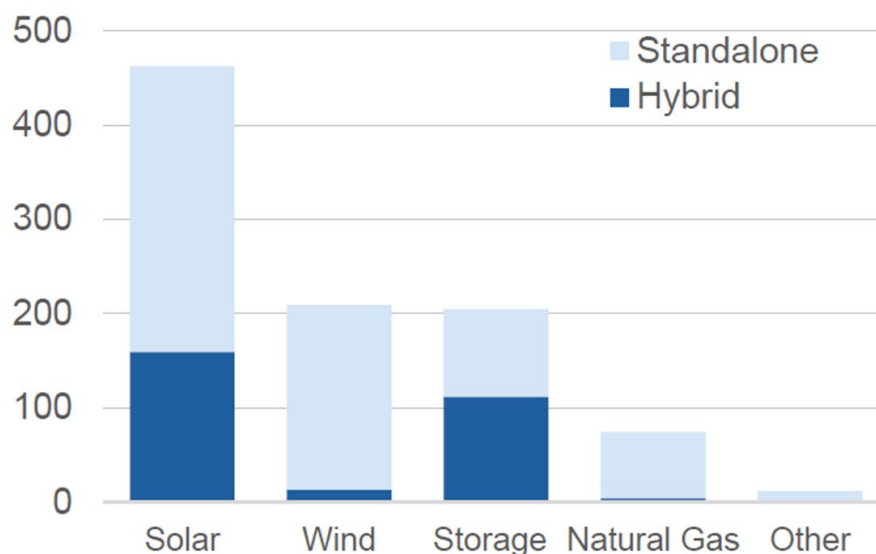
Figure 4.4 – Capacity in U.S. Interconnection Queues (GWs) as of Year-End 2020 42
