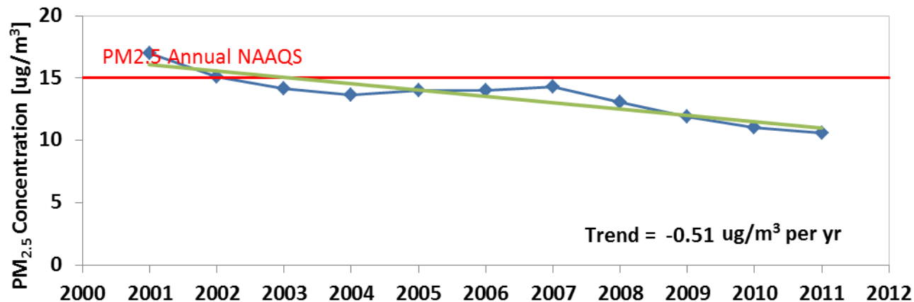
Tennessee Average PM 2.5 Annual Design Values
